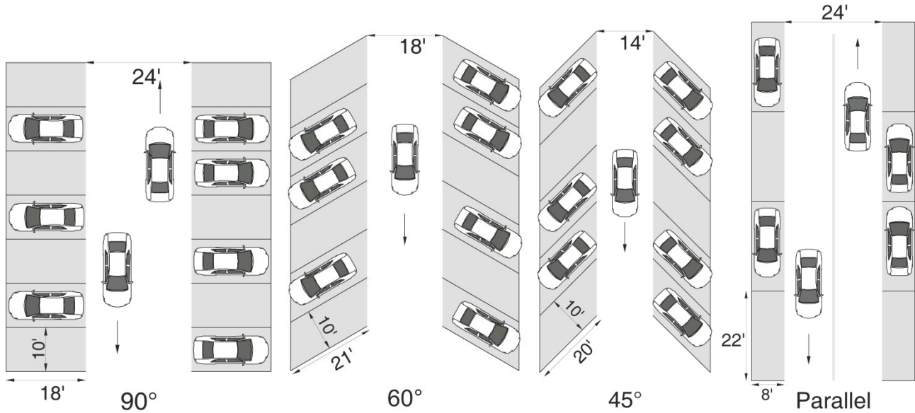
FIGURE 1: Parking Dimensions
